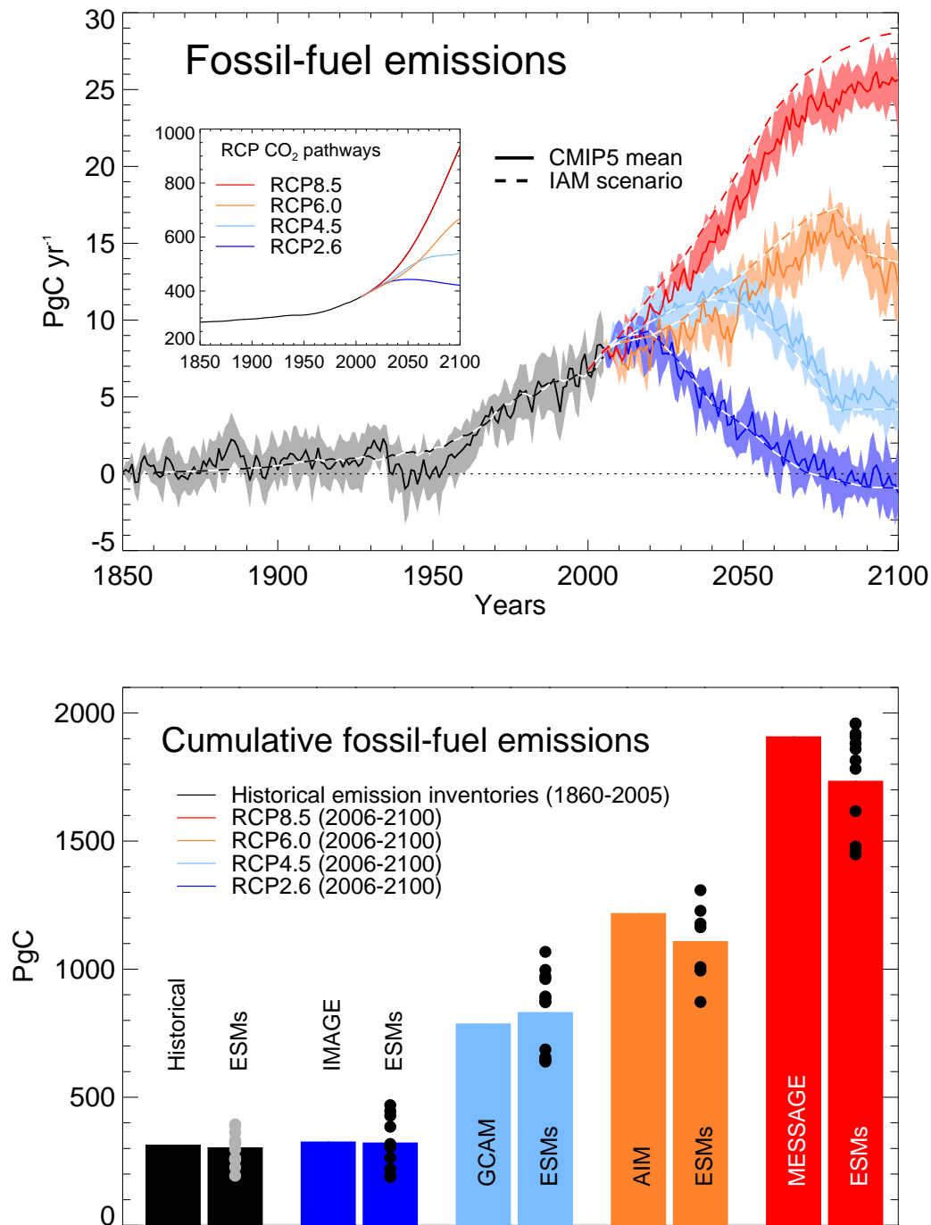
Figure 6.25: Compatible fossil fuel emissions simulated by the CMIP5 ESM models for the 4 RCP scenarios. Top: time series of compatible emission rate ( \text{PgC yr}^{-1} ). Dashed lines represent the historical estimates and emissions calculated by the integrated assessment models (IAM) used to define the RCP scenarios, solid lines and plumes show results from CMIP5 ESMs (model mean, with 1 standard deviation shaded). Bottom: cumulative emissions for the historical period (1860–2005) and 21st century (defined in CMIP5 as 2006–2100) for historical estimates and RCP scenarios. Dots denote individual ESM results, bars show the multi-model mean. In the CMIP5 model results, total carbon in the land-atmosphere-ocean system can be tracked and changes in this total must equal fossil fuel emissions to the system (see Box 6.4). Models used: CanESM2, GFDL-ESM2G, GFDL-ESM2M, HadGEM2-CC, HadGEM2-ES, IPSL-CM5A-LR, IPSL-CM5A-MR, IPSL-CM5B-LR, MIROC-ESM-CHEM, MIROC-ESM, MPI-ESM-LR, NorESM1-ME, INMCM4, CESM1-BGC, BCC-CSM1.1. Not every model performed every scenario simulation.
