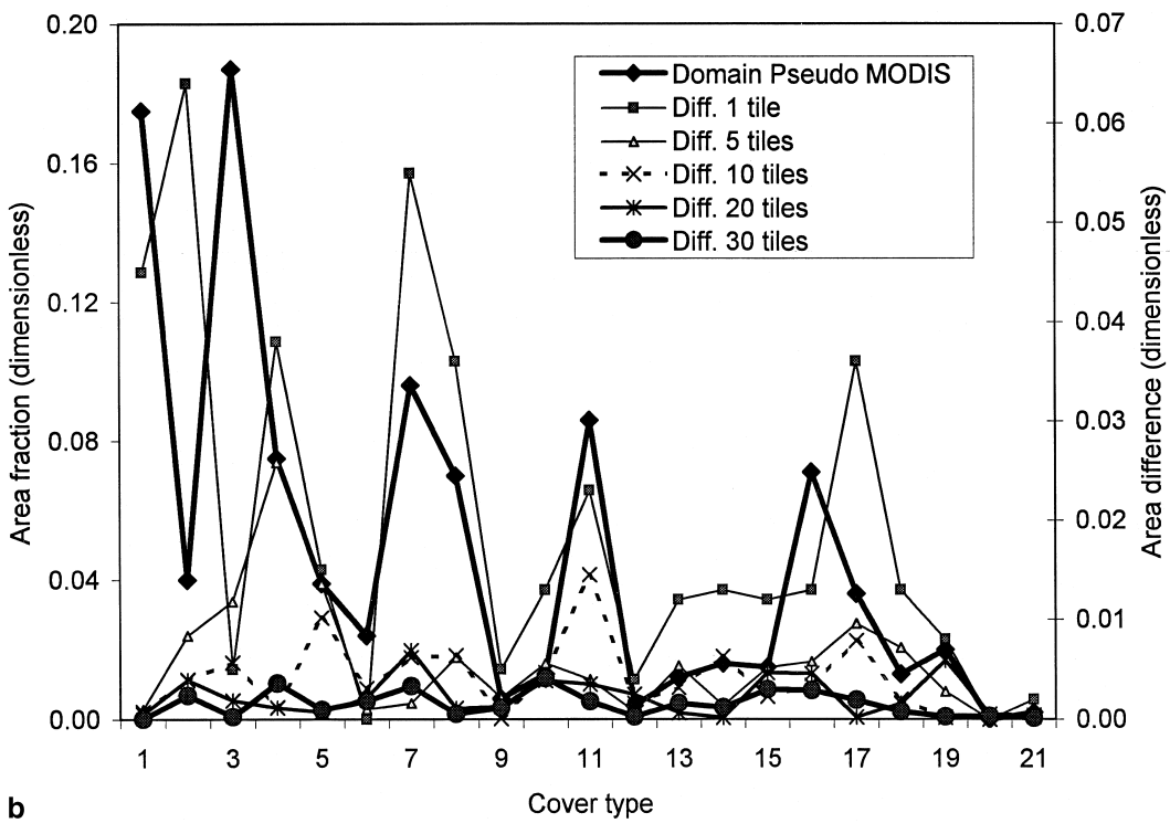
Figure 5. The cover type area fraction and the absolute difference between the fraction of land cover type in the domain map and the sample (right-hand y -axis), for individual cover types: TM (a), P-MODIS (b), AVHRR (c). The difference is computed between the domain values for that date type and the sample.
