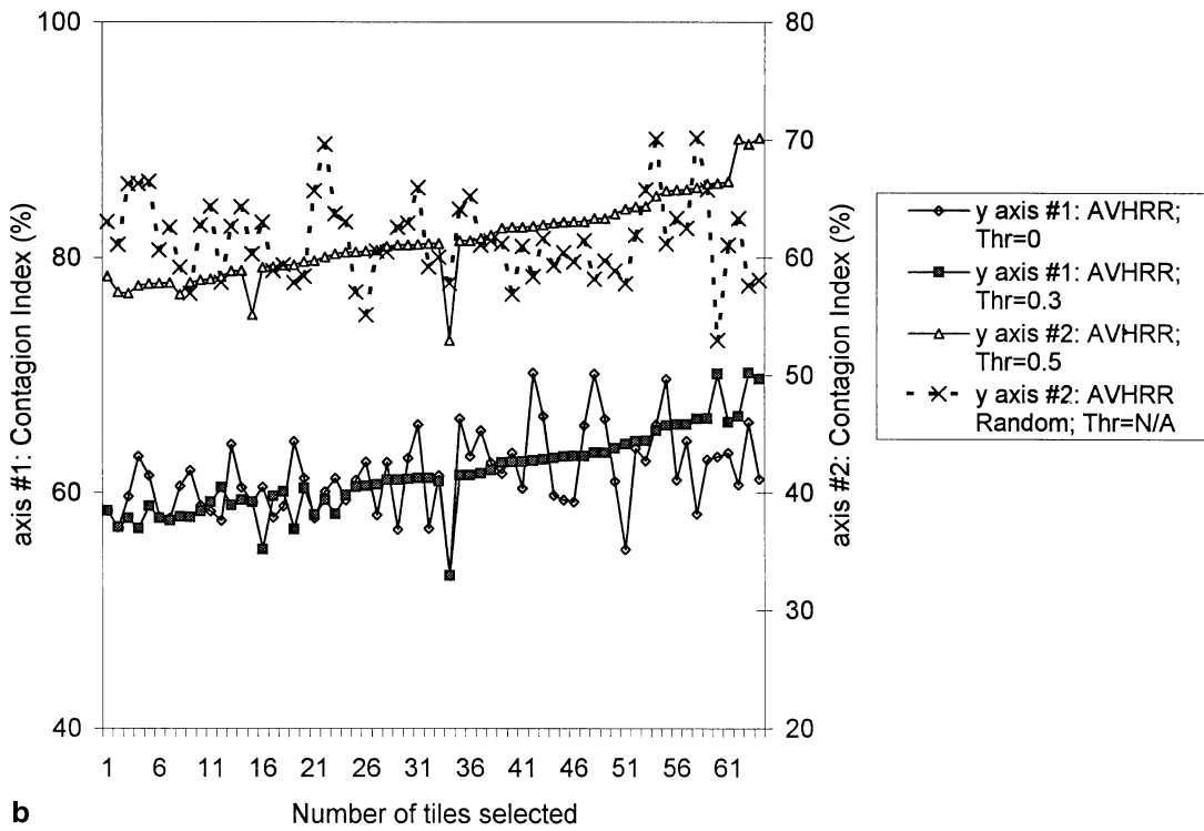
Figure 4. The contagion index (CI) between the domain and the tile selected at each step for various threshold values: TM land cover map (a), AVHRR map (b).
