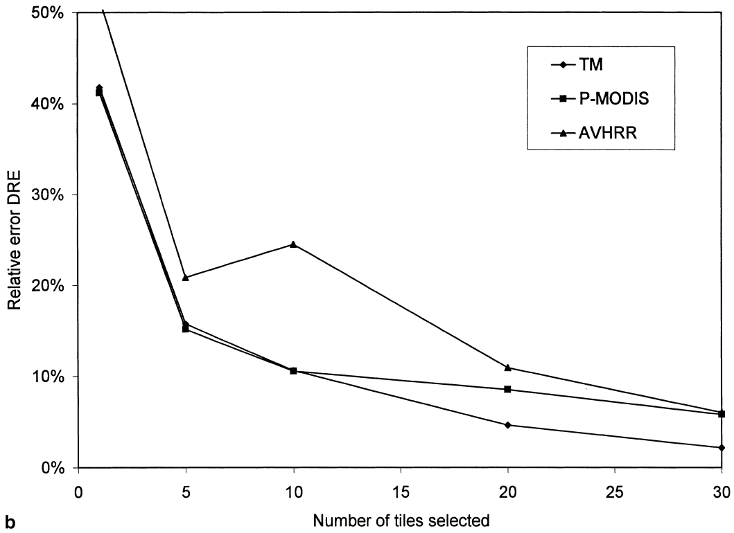
Figure 6. The mean relative error (DRE) between the domain and the selected tiles with different reference data. a) Compared to the domain map of the same data type; b) compared to the TM domain map; c) compared to the TM domain map and without the smallest class (occupying 0.3% of the domain).
