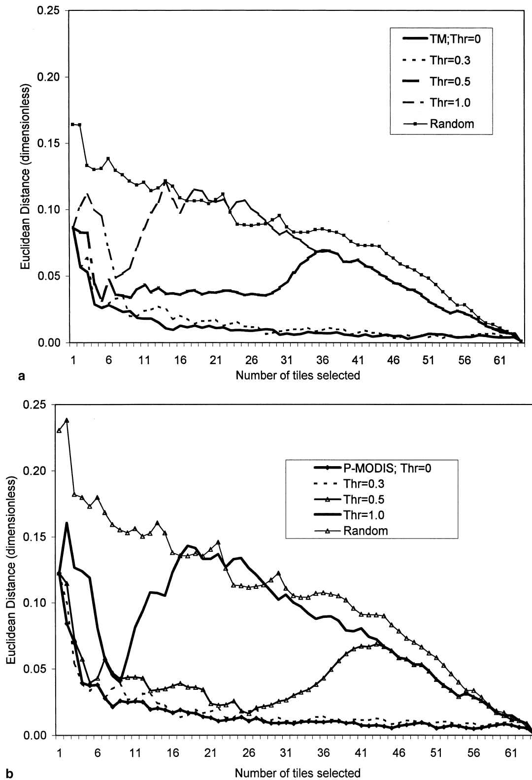
Figure 3. The mean Euclidean distance (ED) between the domain and the tiles selected using various threshold values, and for a random tile selection: TM land cover map (a), P-MODIS map (b), AVHRR map (c).
