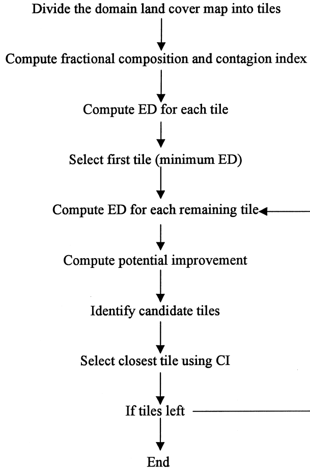
Figure 1. Flowchart of the tile selection algorithm.
