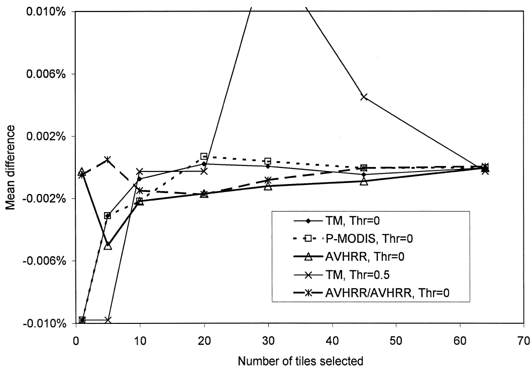
Figure 8. Mean difference (sign considered) between the fraction of the area occupied by a class in the domain and the sample. The reference used is the TM domain map, except for the AVHRR/AVHRR curve where the reference is the AVHRR domain map.
