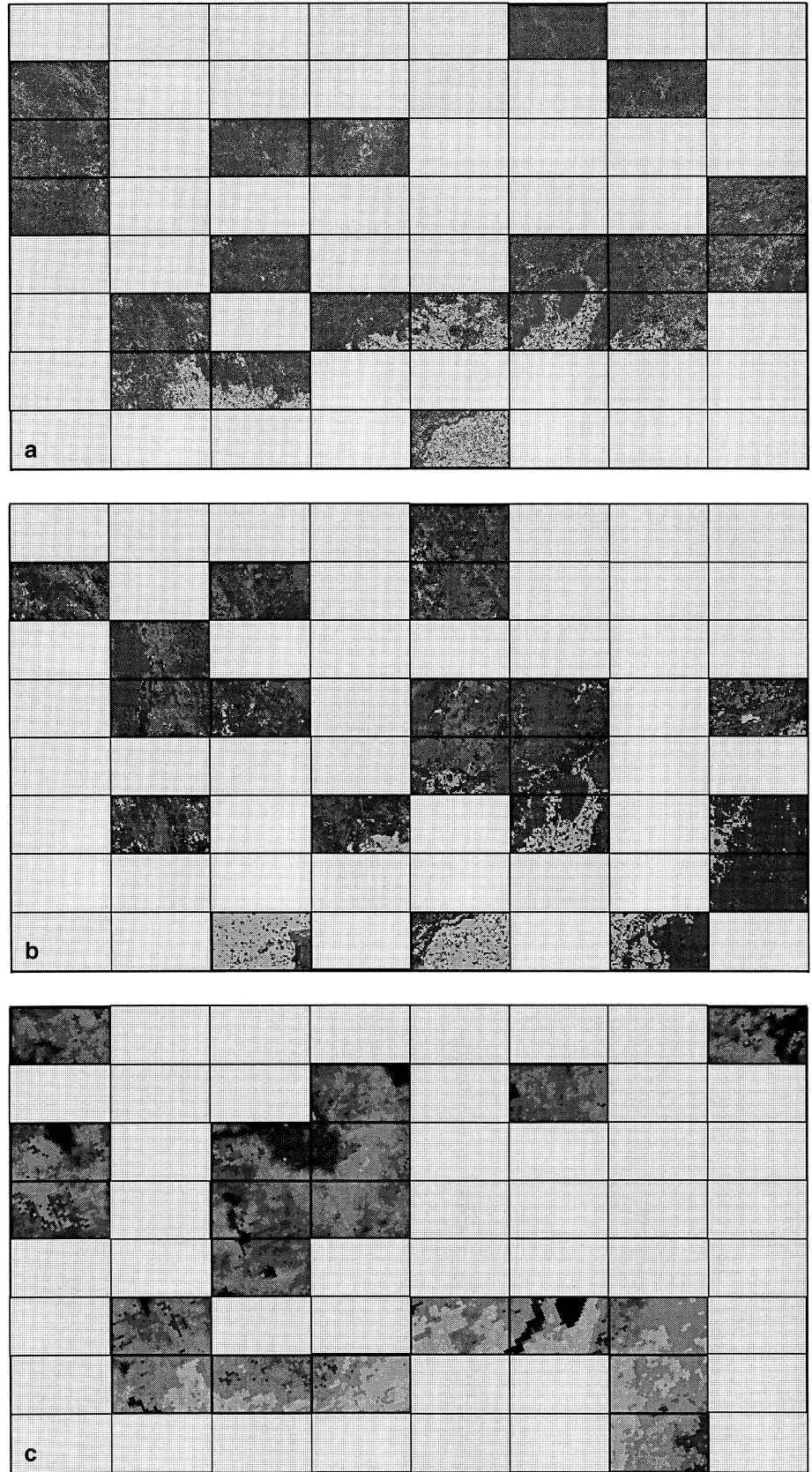
Figure 7. Tiles selected after 20 steps using TM map (a), P-MODIS (b), and AVHRR (c).
