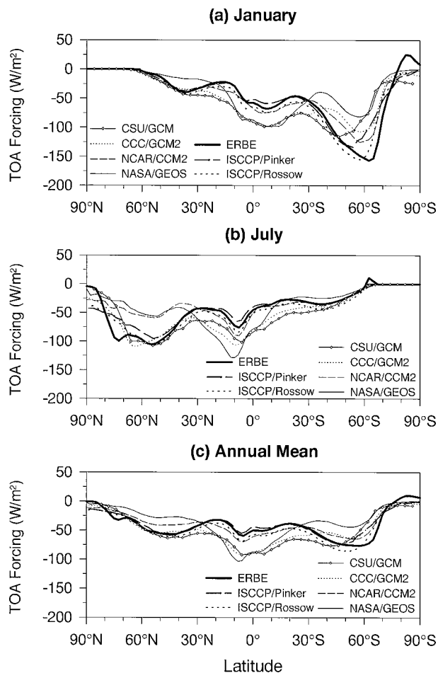
FIG. 4. Comparison of zonal mean cloud radiative forcing at the top of the atmosphere.
